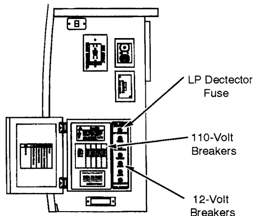
Power Load Center - Model 221RC (On end of vanity cabinet)
