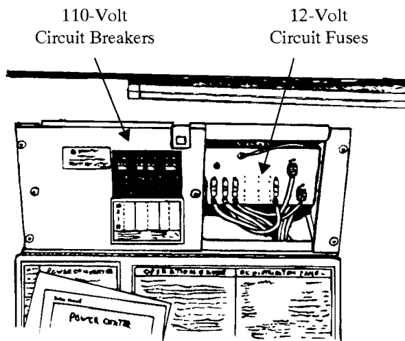
Power Load Center - Model 221RD
