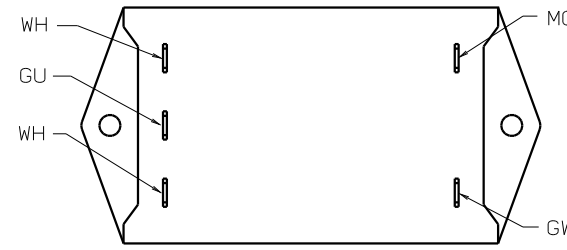
DETAIL AB TOP VIEW
