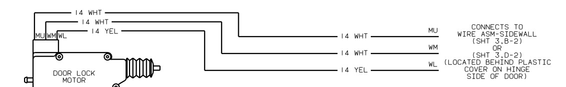
WIRING DIAGRAM-POWER LOCK ENTRANCE (WIRE ASM 93057-04)
