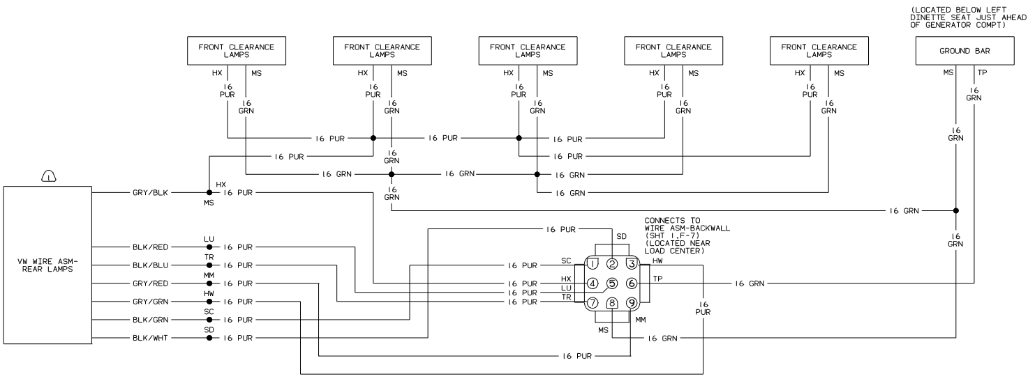
WIRE ASM-CLEARANCE/TAILLAMPS (WIRE ASM 112678)
