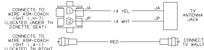
WIRING DIAGRAM-SIDEWALL (WIRE ASM 111451-03)
