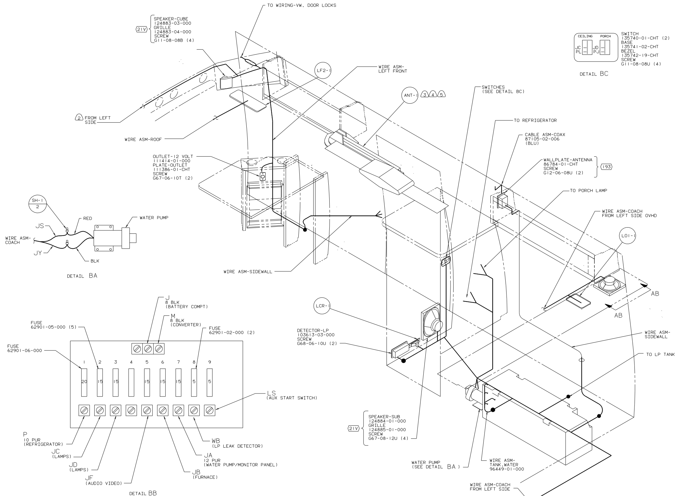
DETAIL BB
