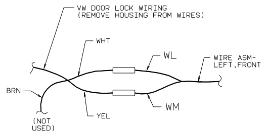
DETAIL BF
