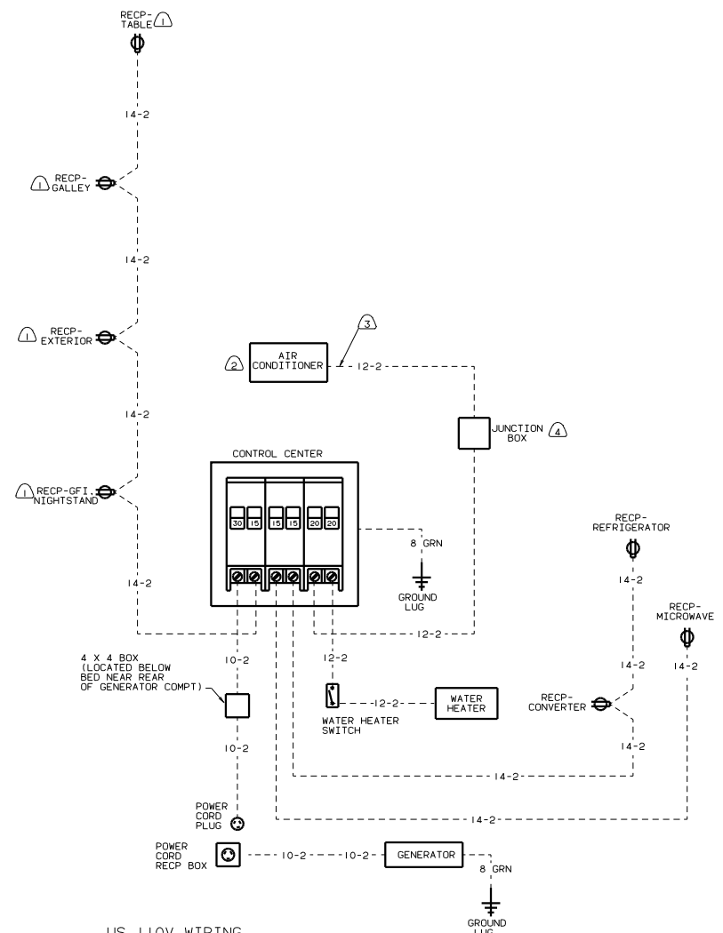
US 110V WIRING (DOUBLE BED) (TWIN BED)
