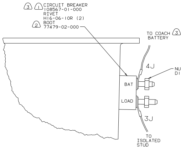
VIEW EE-EE
