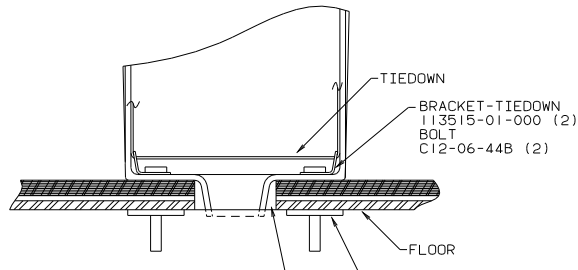
DETAIL EB-EB
