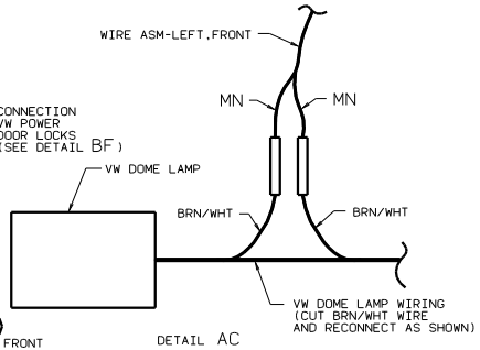
DETAIL AC
