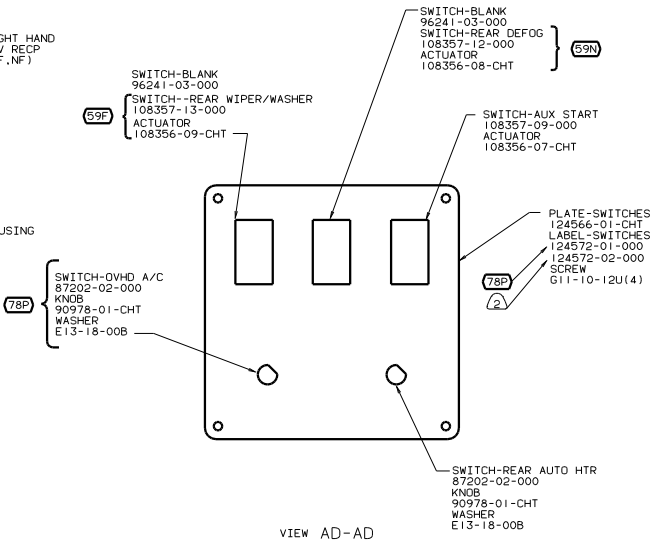
VIEW AD-AD
