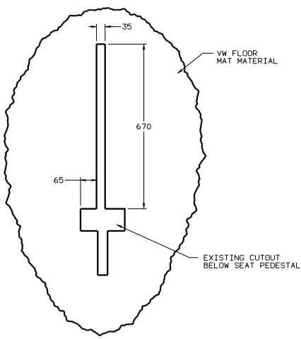
VIEW AA-AA
